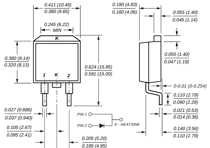
TO-263AB (UGB12 Series)
