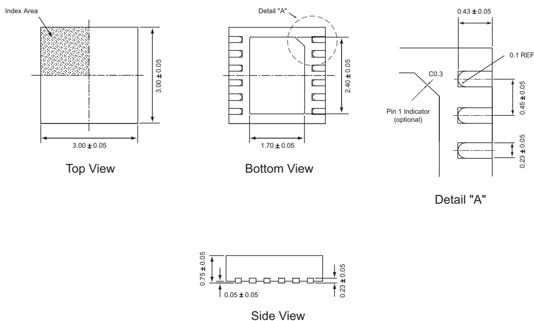
TDFN33-12
