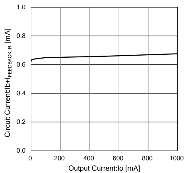
Figure 12. Circuit Current ( I_o=0\text{mA}\rightarrow1000\text{ mA} ) ( I_{FEEDBACK\_R}\cong75\mu\text{A} )
