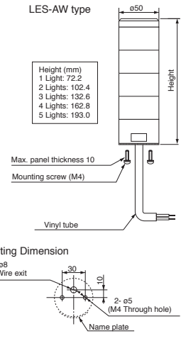
LES-AW type
