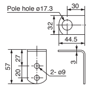
Mounting Dimension
