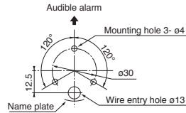
Mounting Dimension
