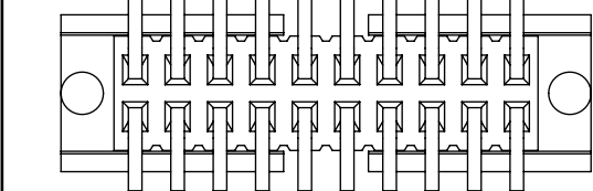
FIG 4 -DV-SA OPTION (SEE NOTES 6 & 7) FTS-106-02-XX-DV-SA SHOWN (DIFFERENT AS SHOWN, OTHERWISE SAME AS FIG 1) NOTE: 4 POSITIONS MUST BE ADDED TO PART CALLOUT TO ACHIEVE DIMS
