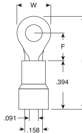
Dimensions: (in.)
