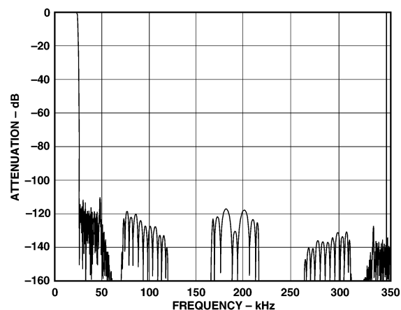
TPC 2. Complete Response, 8 \times Mode, 48 kHz Sample Rate
