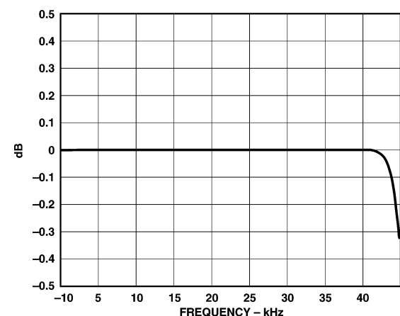
TPC 3. 44 kHz Pass-Band Response 4 \times Mode, 96 kHz Sample Rate
