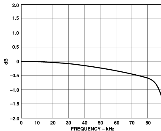
TPC 5. Pass-Band Response, 2 \times Mode, 192 kHz Sample Rate
