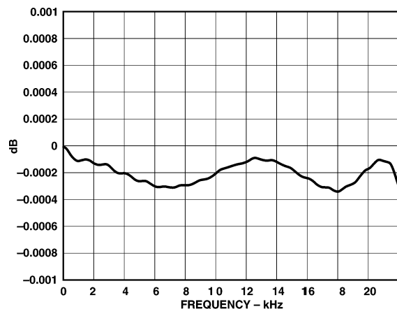
TPC 1. Pass-Band Response, 8 \times Mode, 48 kHz Sample Rate
