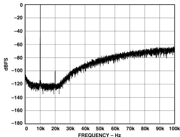
TPC 32. Wideband FFT Plot, 64 \times f_s DSD, SR = 44.1 kHz, 0 dBFS @ 10 kHz
