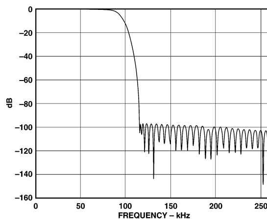
TPC 6. Complete Response, 2 \times Mode, 192 kHz Sample Rate
