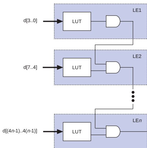
Figure 5. FLEX 8000 Cascade Chain Operation
