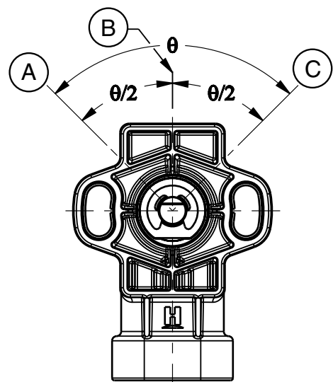
Figure 2. Mounting Dimensions (For Reference only: mm/[in].)
