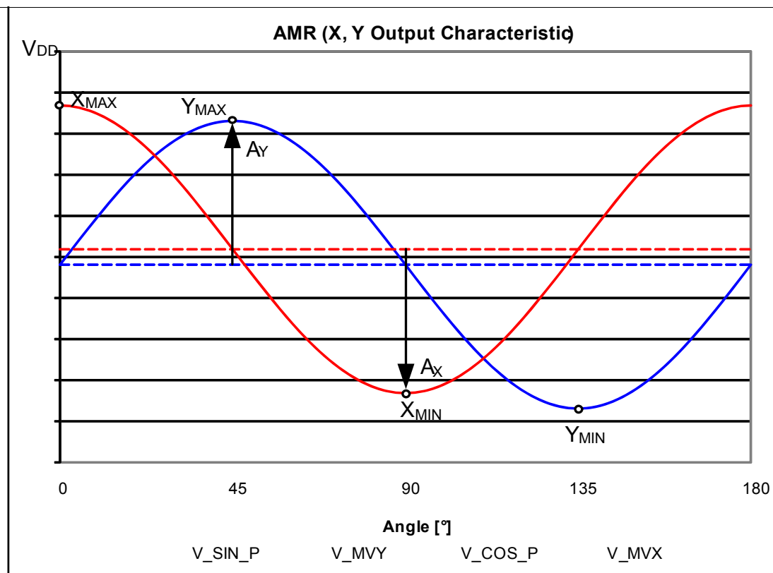
Figure 13 AMR sensor single-ended output signals
