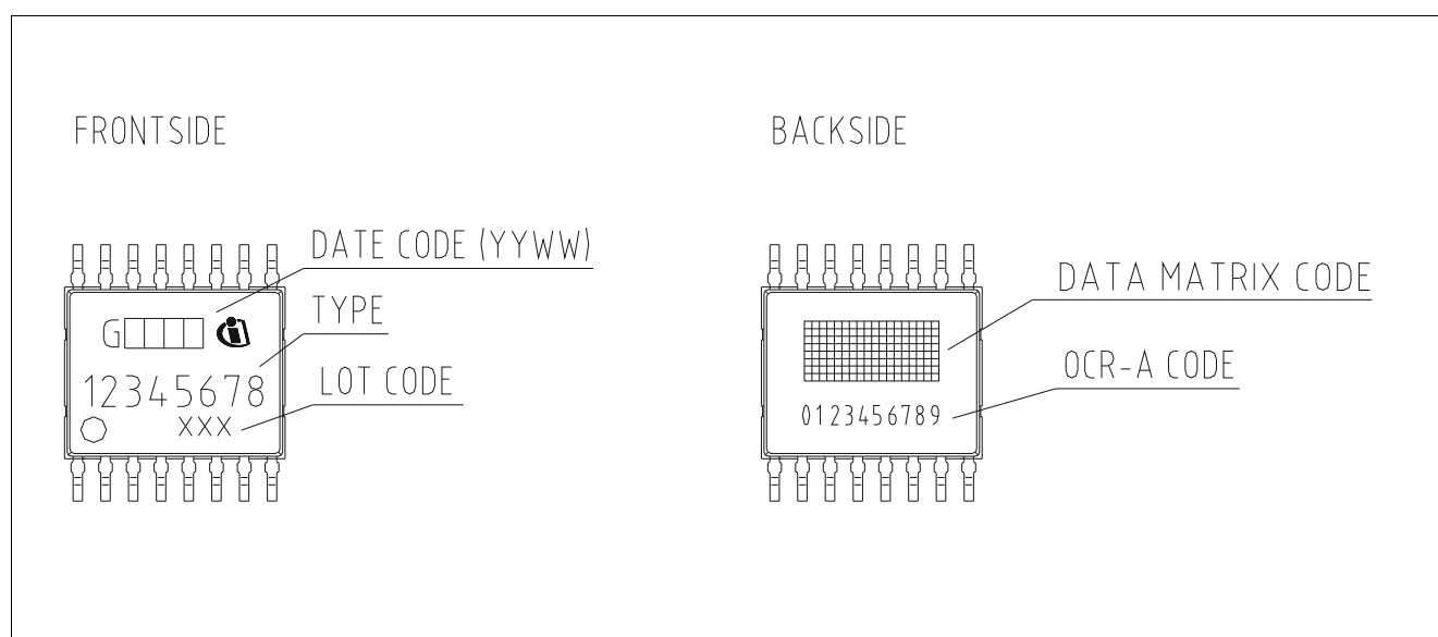
Figure 20 Marking
