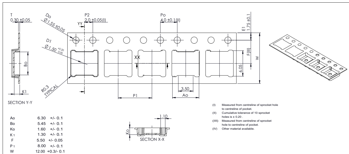
Figure 19 Tape and reel
