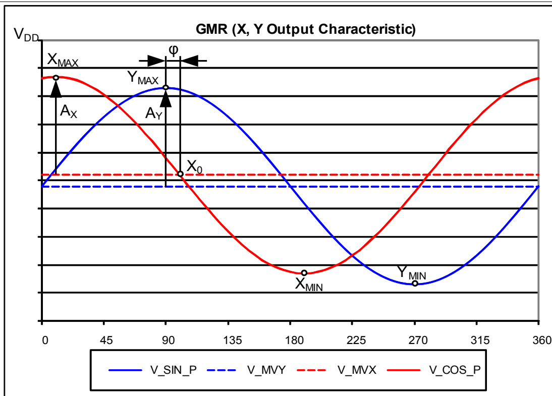
Figure 12 GMR sensor single-ended output signals
