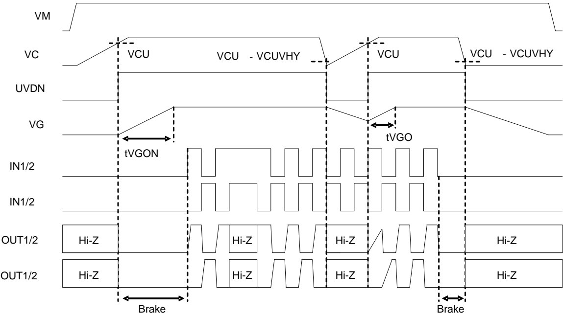
Figure 4. Time chart of input and output (in cace of VDUV detection)
