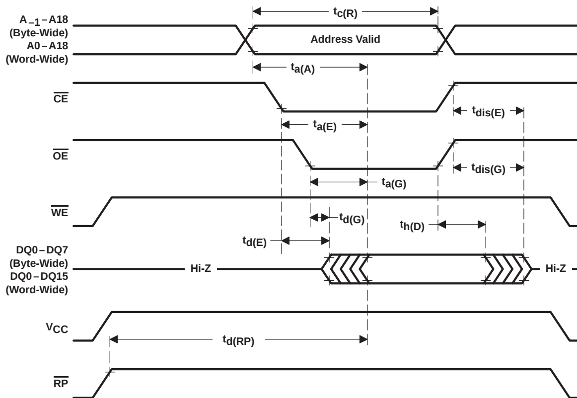
Figure 12. Read-Cycle Timing
