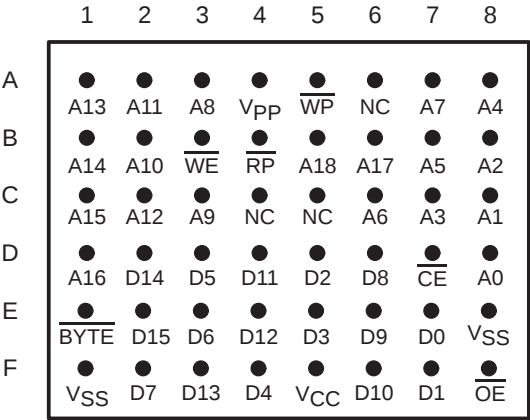
TMS28F800Axy 48-BALL μBGA (TOP VIEW)
