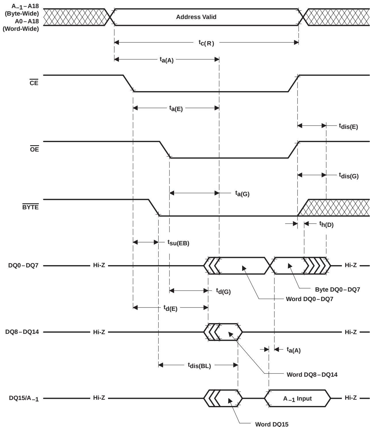
Figure 17. BYTE Timing, Changing From Word-Wide to Byte-Wide Mode
