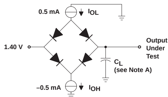
Figure 9. 3-V Testing Load Circuit and Voltage Waveform
