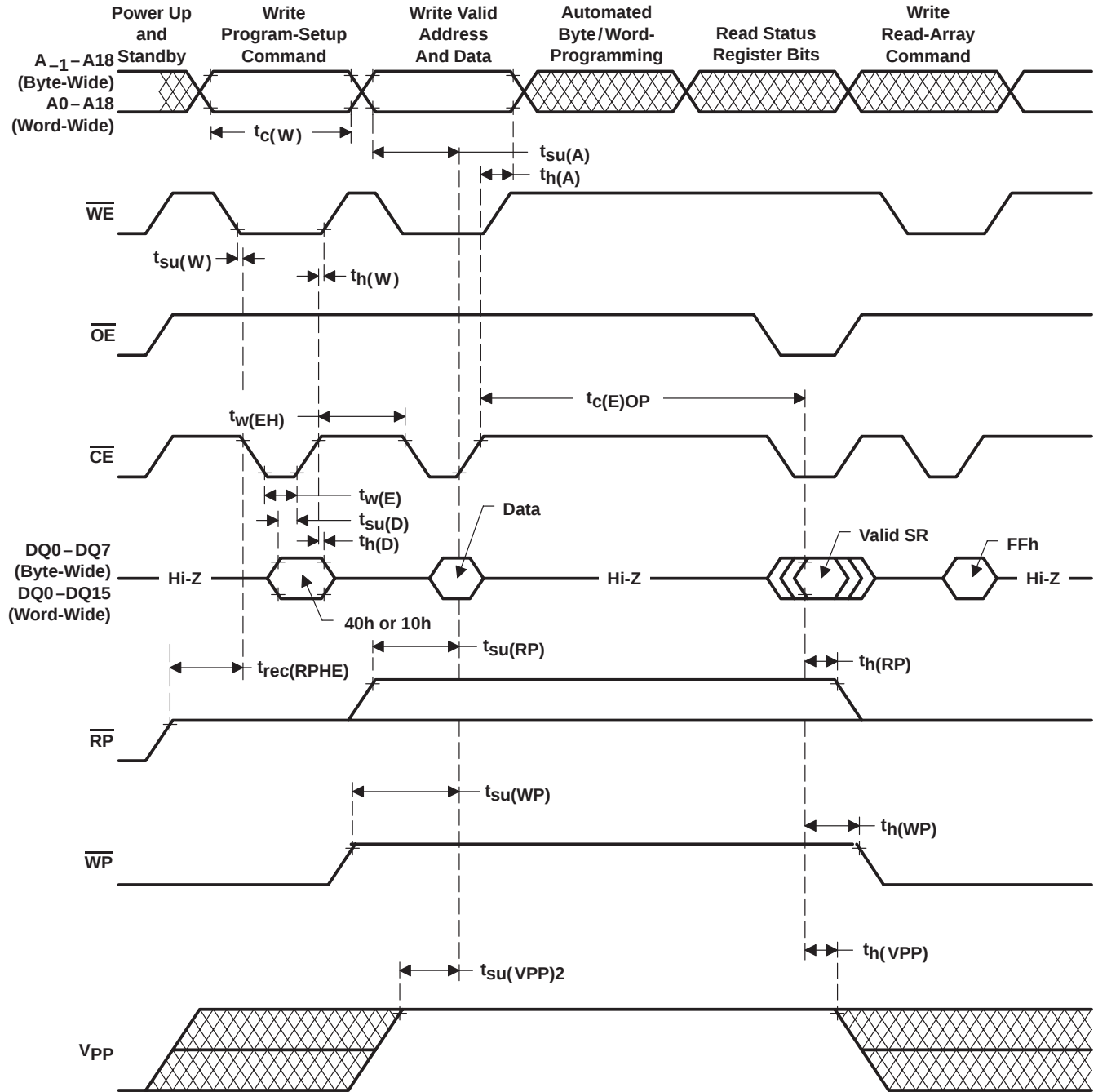
Figure 14. Write-Cycle Timing ( \overline{\text{CE}} -Controlled Write)
