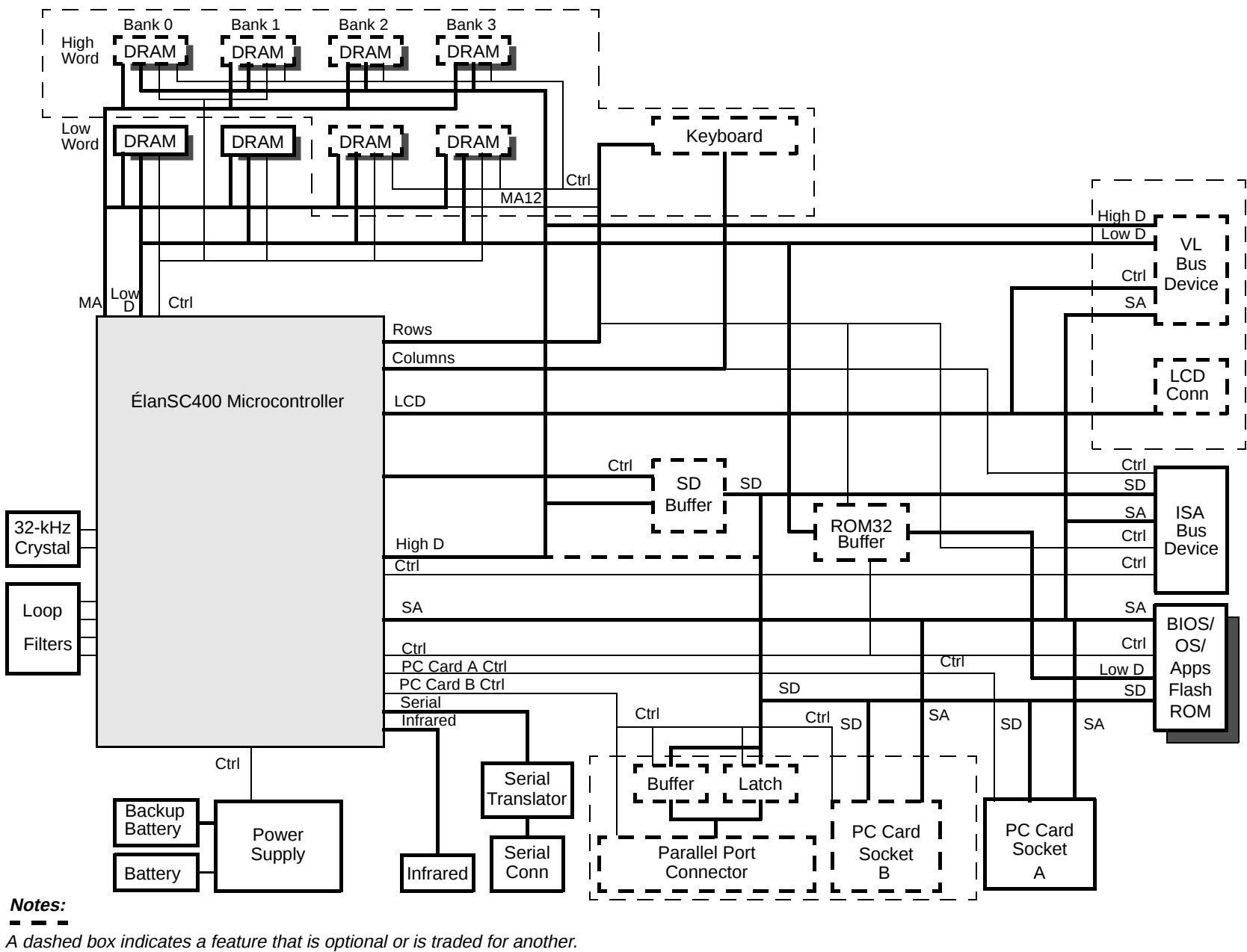
Figure 2. System Diagram with Trade-offs—ÉlanSC400 Microcontroller
