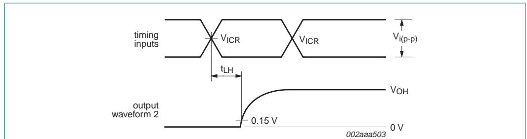
Fig 23. Voltage waveforms, open-drain output LOW-to-HIGH transition time with respect to clock inputs
