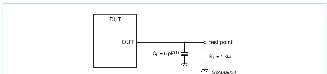
Fig 24. Partial parity out load circuit
