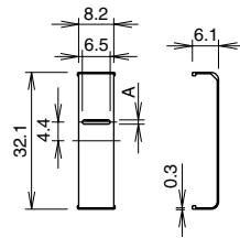
Horizontal Slit
