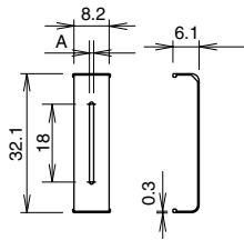
Vertical Slit
