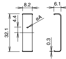
Round Slit
