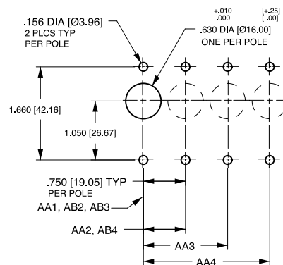
PANEL CUTOUT DETAIL
