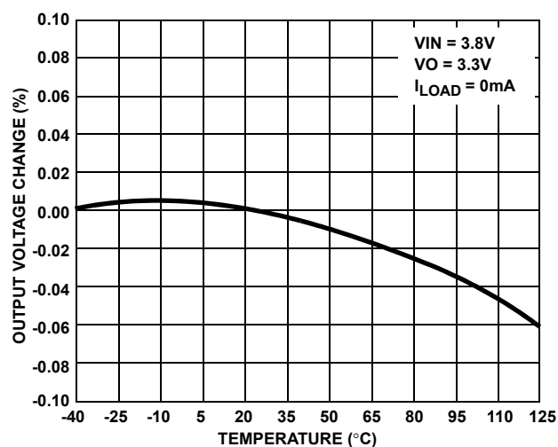
FIGURE 4. OUTPUT VOLTAGE CHANGE vs TEMPERATURE
