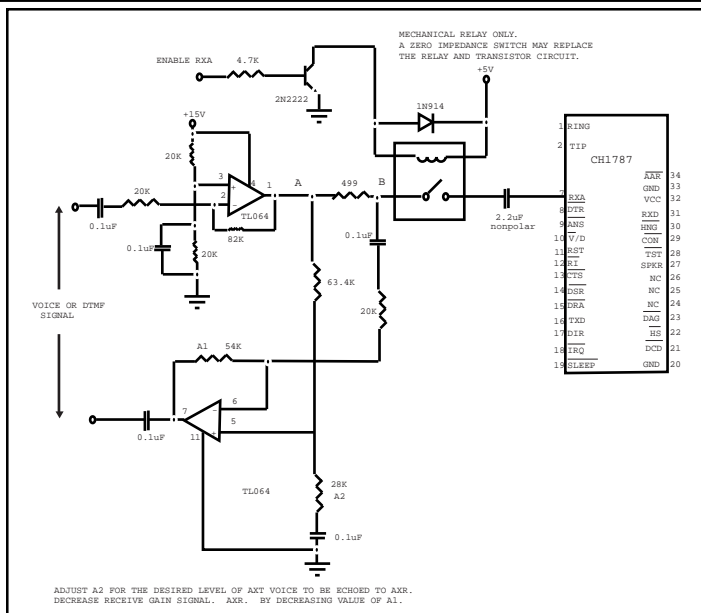
Figure 3. Voice/Tone Injection
