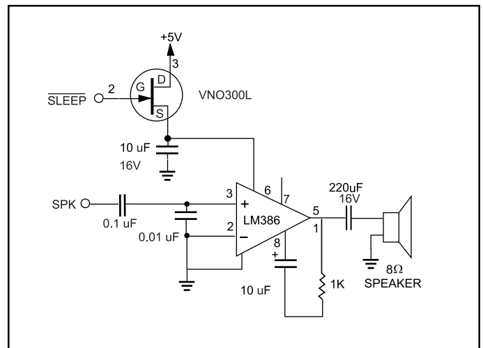
Figure 5. Speaker Control Circuit--optional to allow for call progress monitoring.
