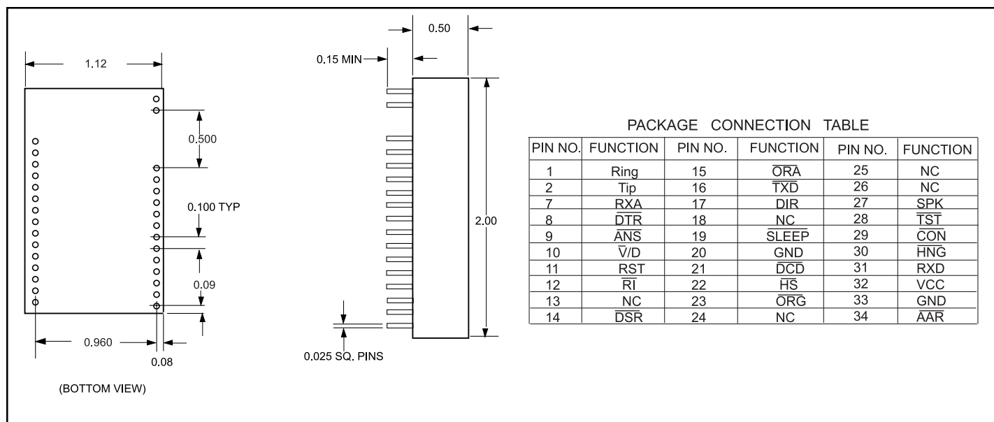
Figure 7. CH1787 Physical Dimensions and Pin Functions
