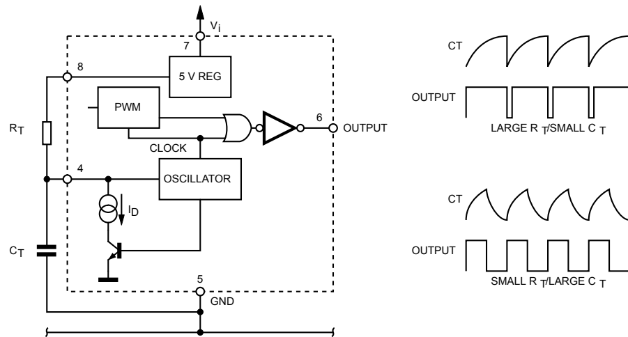
Figure 16. Oscillator and output waveforms
