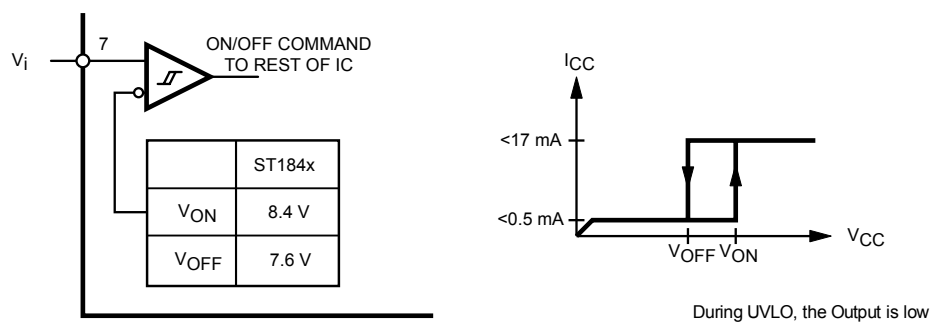
Figure 18. Undervoltage lockout
