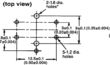
PCB mounting (top view)
