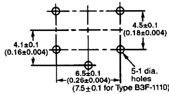
PCB mounting (top view)
