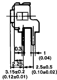
PCB mounting (top view)
