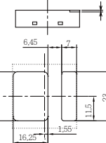
Soldering patterns
