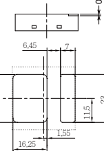
Soldering patterns
