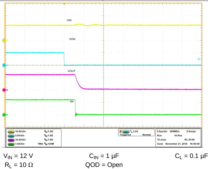
Figure 15. Fall Time t_F at V_{IN} = 12\text{ V}
