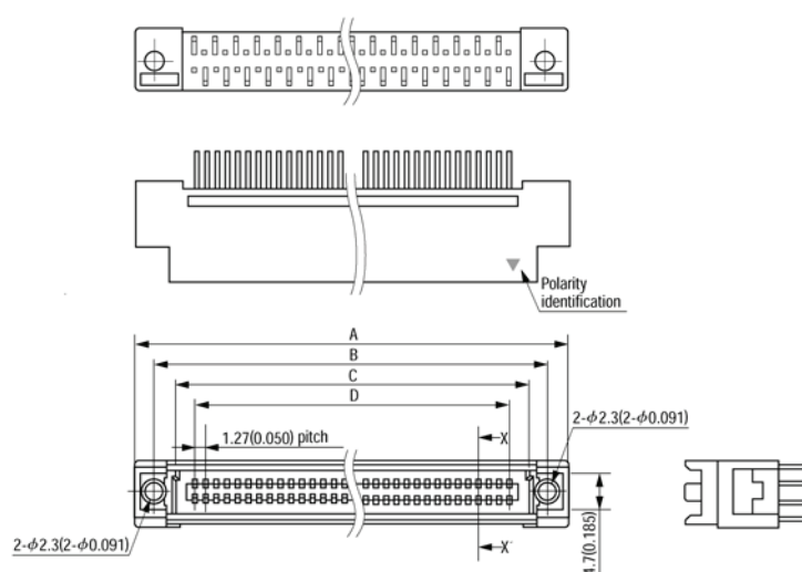
Straight Plug
