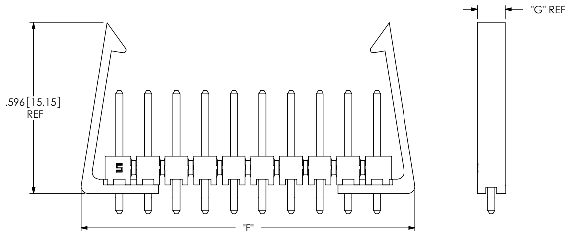
FIG 2: LOCKING CLIP HTSW-T10-07-XXX-D-LC SHOWN (DIFFERENT AS SHOWN, OTHERWISE SAME AS FIG 1)
