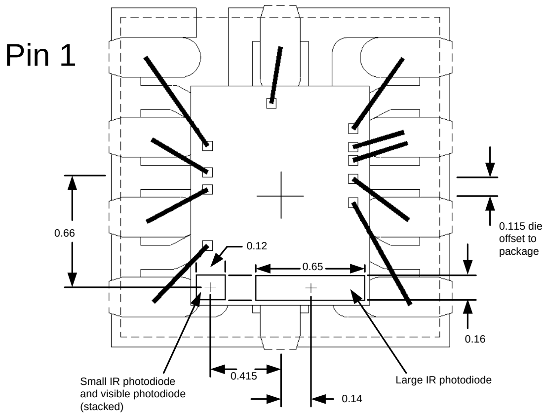
Figure 20. Photodiode Centers
