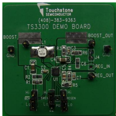
Figure 1. TS3300 Demo Board (Top View)
