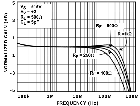
FIGURE 12. GAIN vs FREQUENCY FOR VARIOUS R_{\text{FEEDBACK}} ( A_V = +2 )
