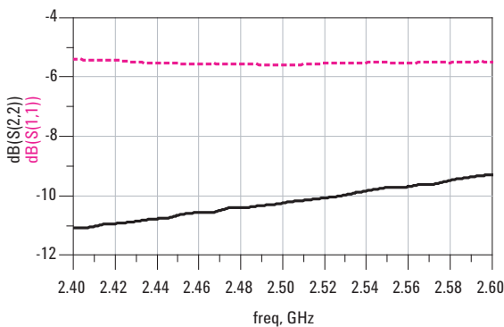
Figure 14. Typical Scattering Parameter Plots
