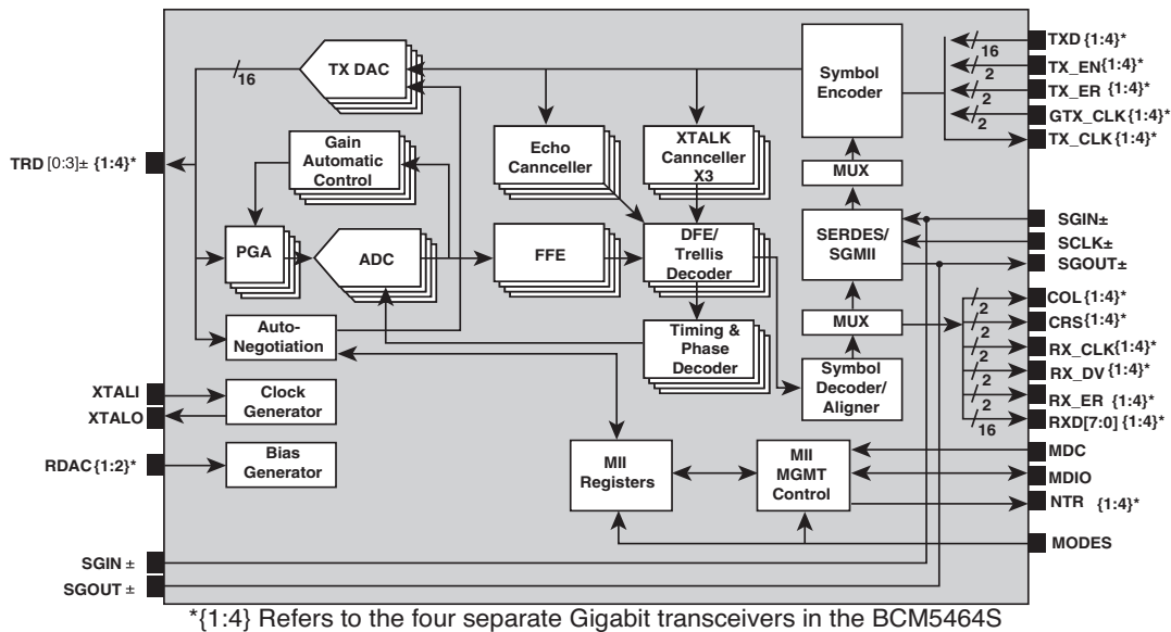
BCM5464S Block Diagram
