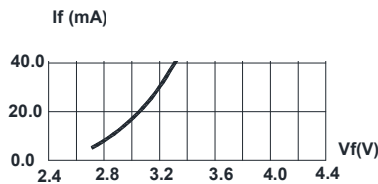
FIG.1 FORWARD CURRENT VS. FORWARD VOLTAGE.
