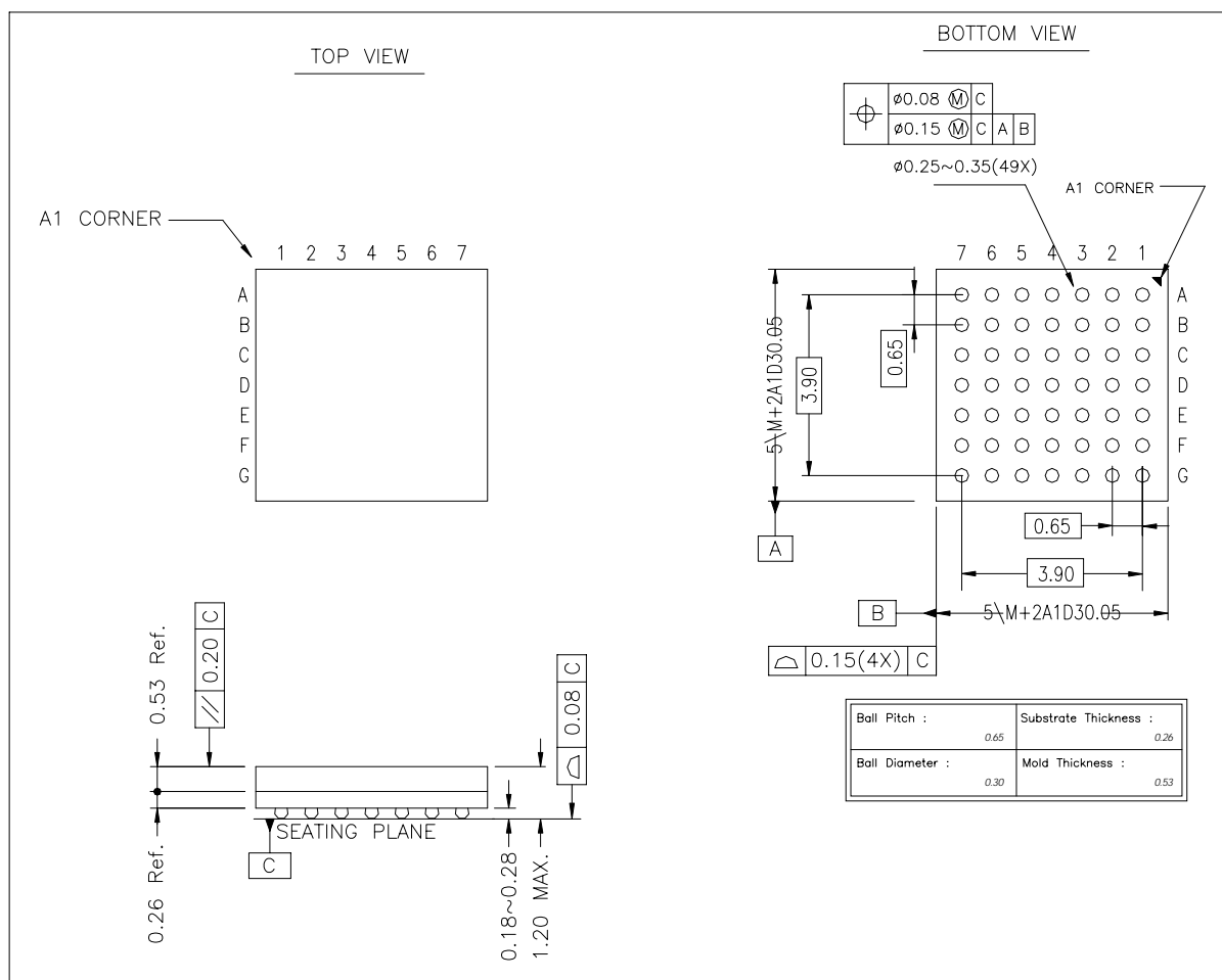
Figure 10. Mechanical Package Drawing for 49-ball Ball Grid Array
