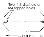
Mounting Holes
