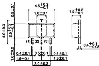
2SB1188
