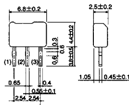
2SB911M
