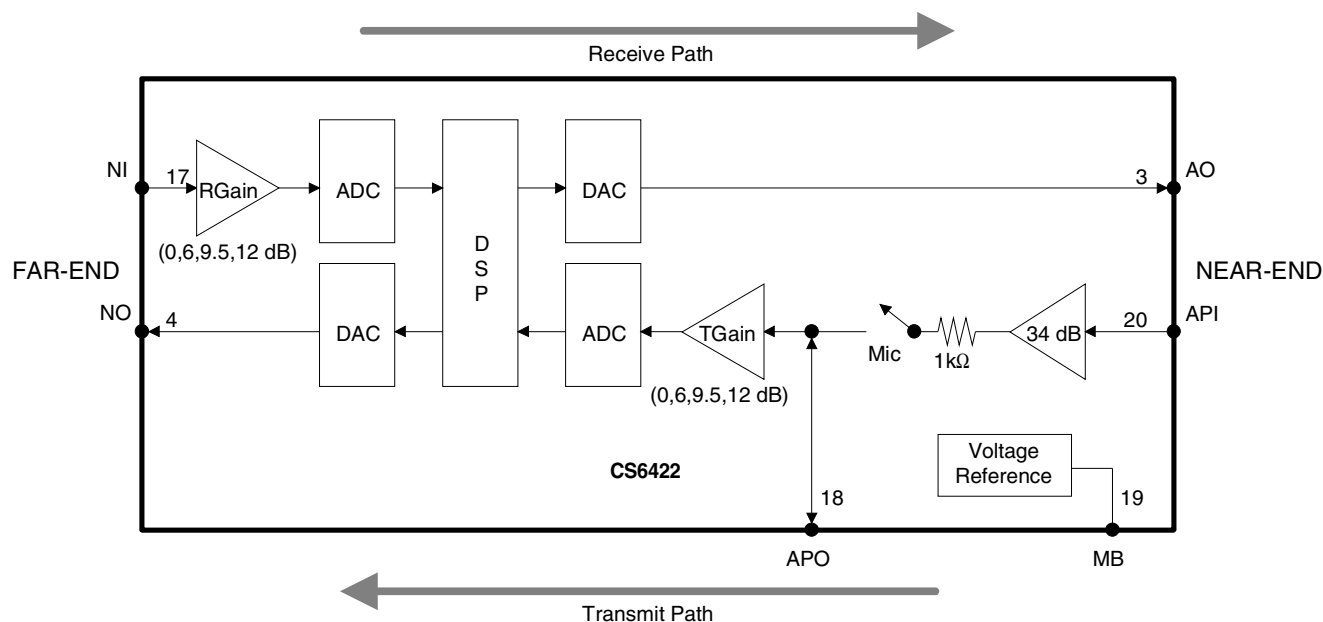
Figure 6. Analog Interface
