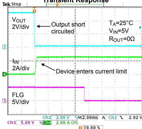
No-Load to Short-Circuit Transient Response
