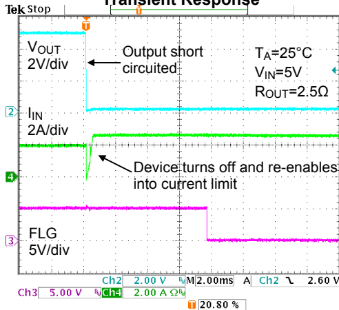
Full-Load to Short-Circuit Transient Response
