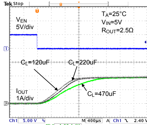
Inrush Current
