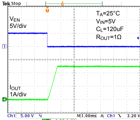
Device Enabled Into Short-Circuit
