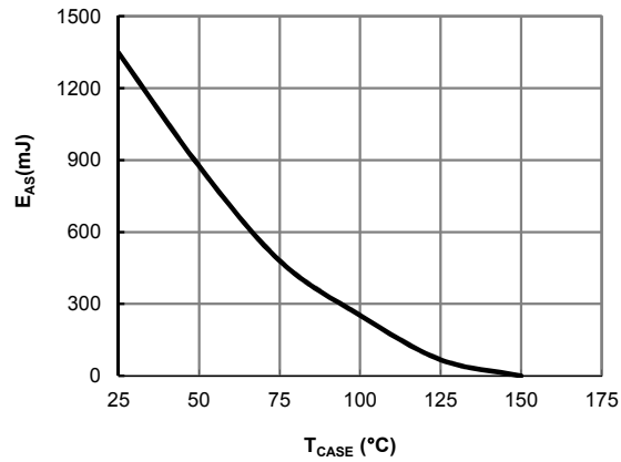
Figure 12: Avalanche energy
