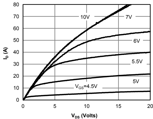
Figure 1: On-Region Characteristics@25°C
