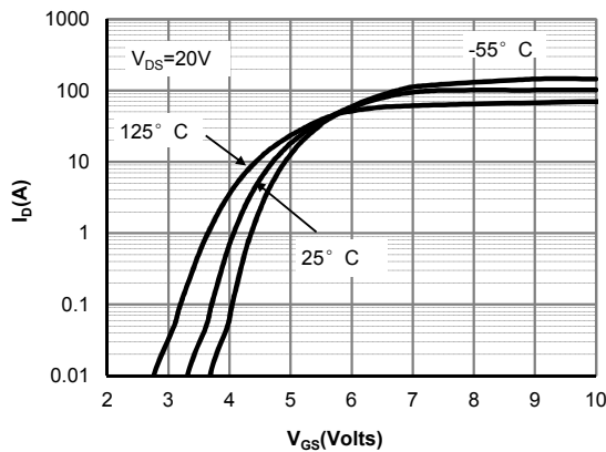
Figure 3: Transfer Characteristics
