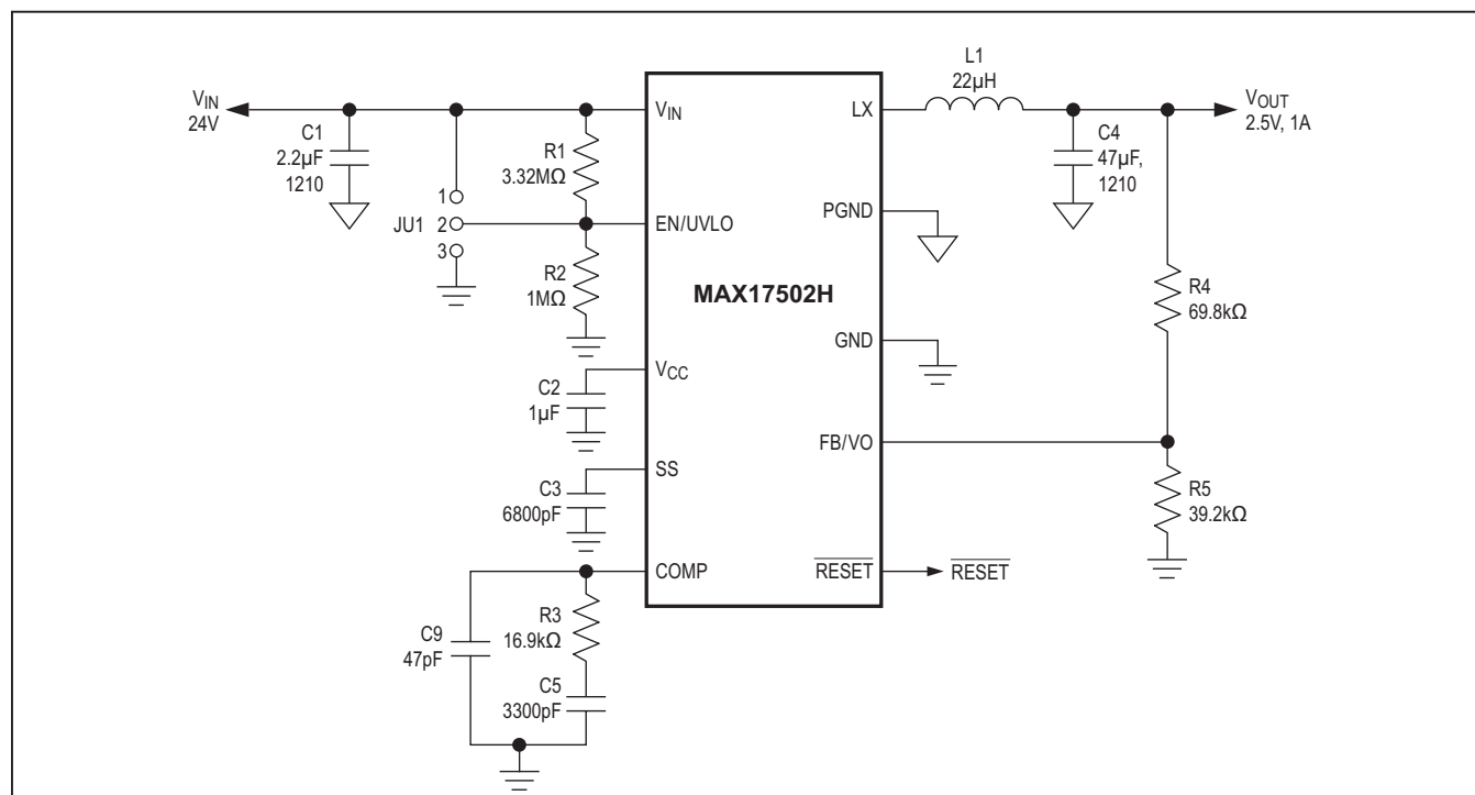
Figure 10. MAX17502H Application Circuit (2.5V Output, 1A Maximum Load Current, 300kHz Switching Frequency)
