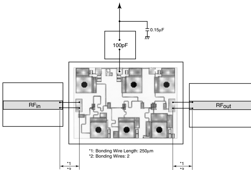
ASSEMBLY DRAWING
