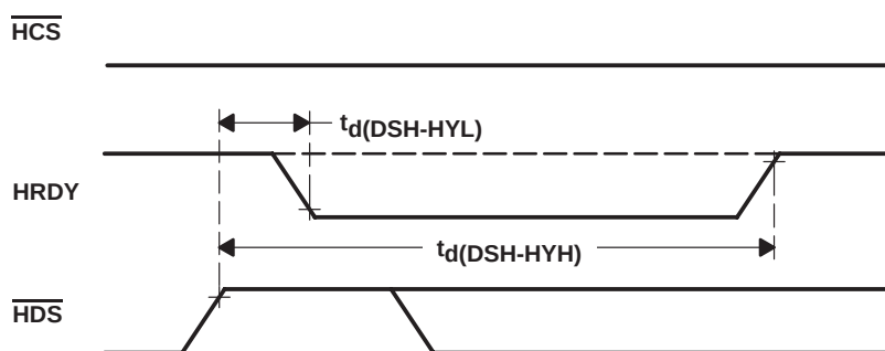
Figure 33. \text{HRDY} Signal When \overline{\text{HCS}} Is Always Low
