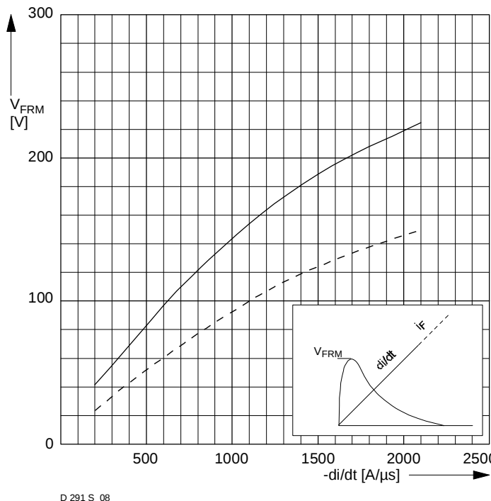
Fig. 4 Peak forward recovery voltage (typical values)
