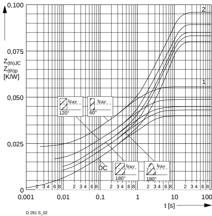
Fig. 2 Transient thermal impedance DC and impuls current ( f = 50\text{ Hz} ) Parameter: Current wave form
