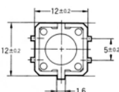
PCB Mounting (Top View) (Single-sided PCB, t=1.6 ) Two, 1.8 \pm 0.05 dia. (For positioning boss)
