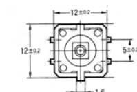
PCB Mounting (Top View) (Single-sided PCB, t=1.6 ) Two, 1.8 \pm 0.05 dia. (For positioning boss)
