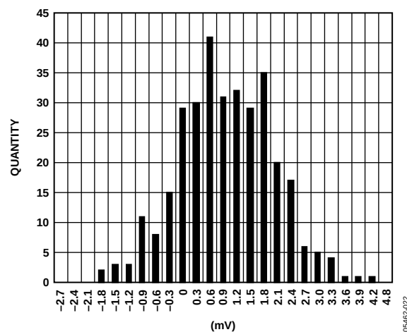
Figure 22. DAC Offset Distribution at 25°C/3.3 V
