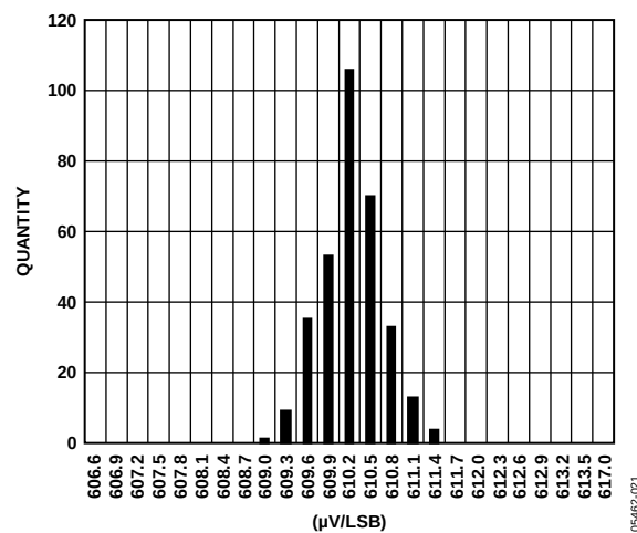
Figure 21. DAC Gain Distribution at 25°C/3.3 V
