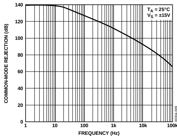
Figure 9. Common-Mode Rejection vs. Frequency
