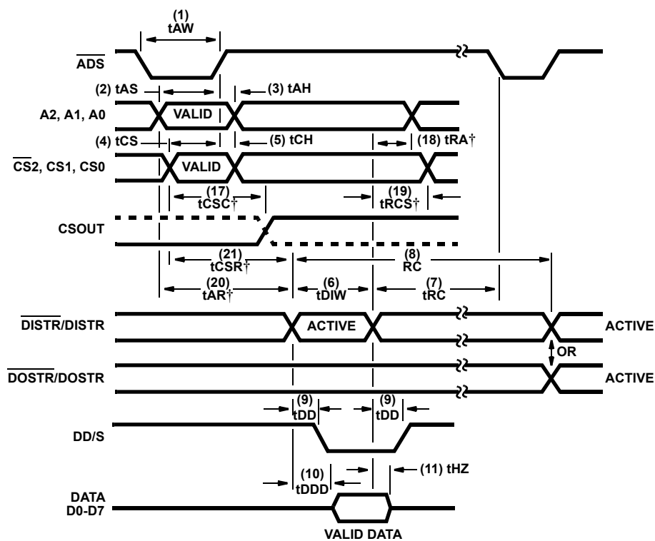
FIGURE 7. READ CYCLE
