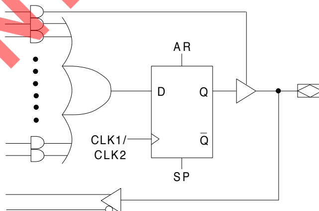
ACTIVE HIGH REGISTERED OUTPUT WITH I/O FEEDBACK
