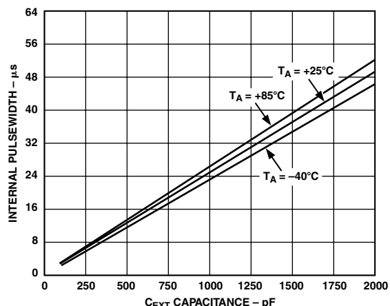
Figure 7. Internal Pulsewidth vs. C EXT
