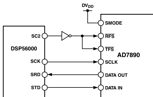
Figure 15. AD7890 to DSP56000 Interface
