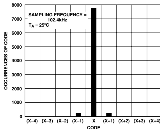
Figure 19. Histogram of 8192 Conversions with Write During Conversion
