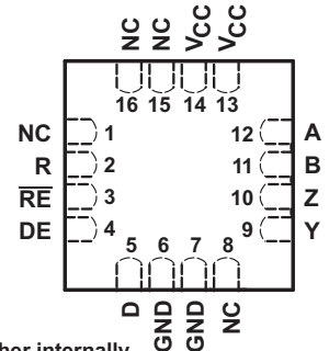
RSA PACKAGE (TOP VIEW)
