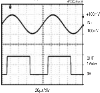
1kHz FREQUENCY RESPONSE ( V_{CC} = 1.8V )
