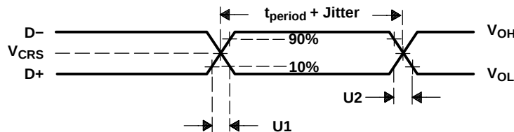
Figure 5–41. USB Timings
