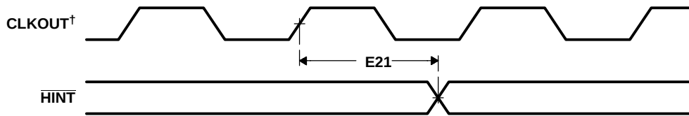
Figure 5–31. \overline{\text{HINT}} Timings
