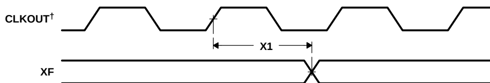
Figure 5–20. XF Timings
