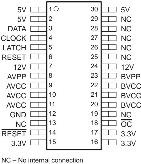
Figure 6. TPS2206 Terminal Assignments
