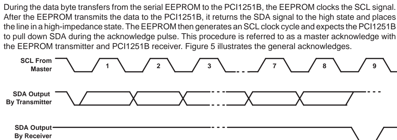
Figure 5. Serial EEPROM Protocol – Acknowledge
